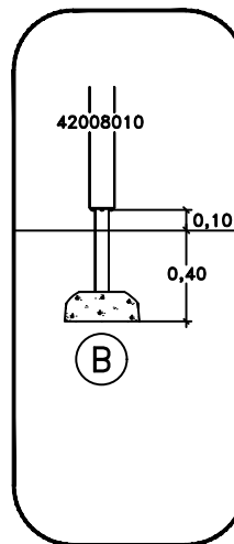
Sunken Foundation
